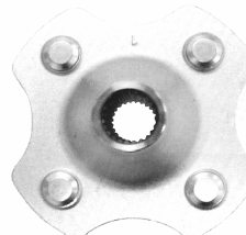
4-Bolt Cast Hub 4 on 150mm 24 Spline CP # 25033
