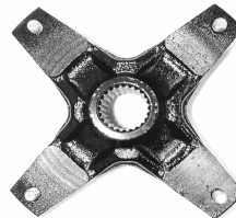
4-Bolt Cast Hub 4 on 150mm 24 Spline CP # 25033
