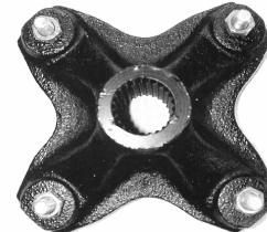
4-Bolt Cast Hub 4 on 130mm 24 Spline CP # 21194
