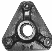
3-Bolt Cast Hub 3 on 100mm 24 Spline CP # 21193
