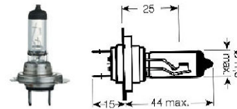
14432 (H7) 12V 55W 14433 (H7) 12V 100W
