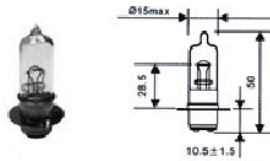
14470 HALOGEN 6V 25/25W 14471 HALOGEN 12V 25/36.5W
