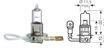
14454 H3 PK22s 12V55W 14458 H3 PK22s 12V100W
