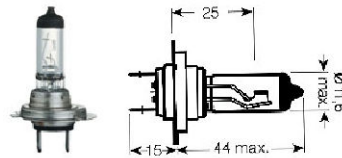
14432 (H7) 12V 55W
