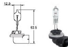
14475 (886) Blue 50w P13t
