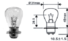
14449-GC 12V-45/45W Fits Golf Car's
