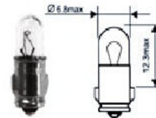
14411 12V-2W BA7S
